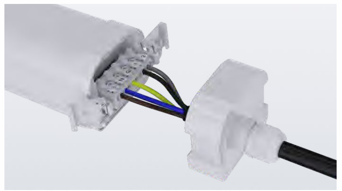
5-core Terminal
