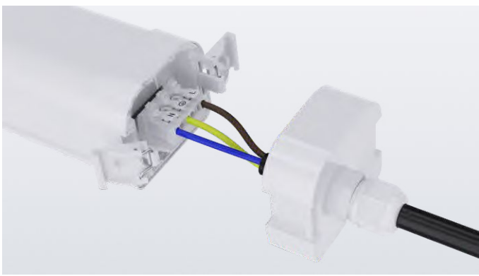
3-core Terminal
